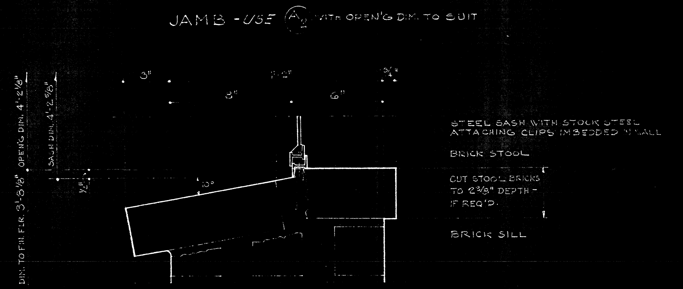
SILL SCALE - 3/8" = 1'-0"
