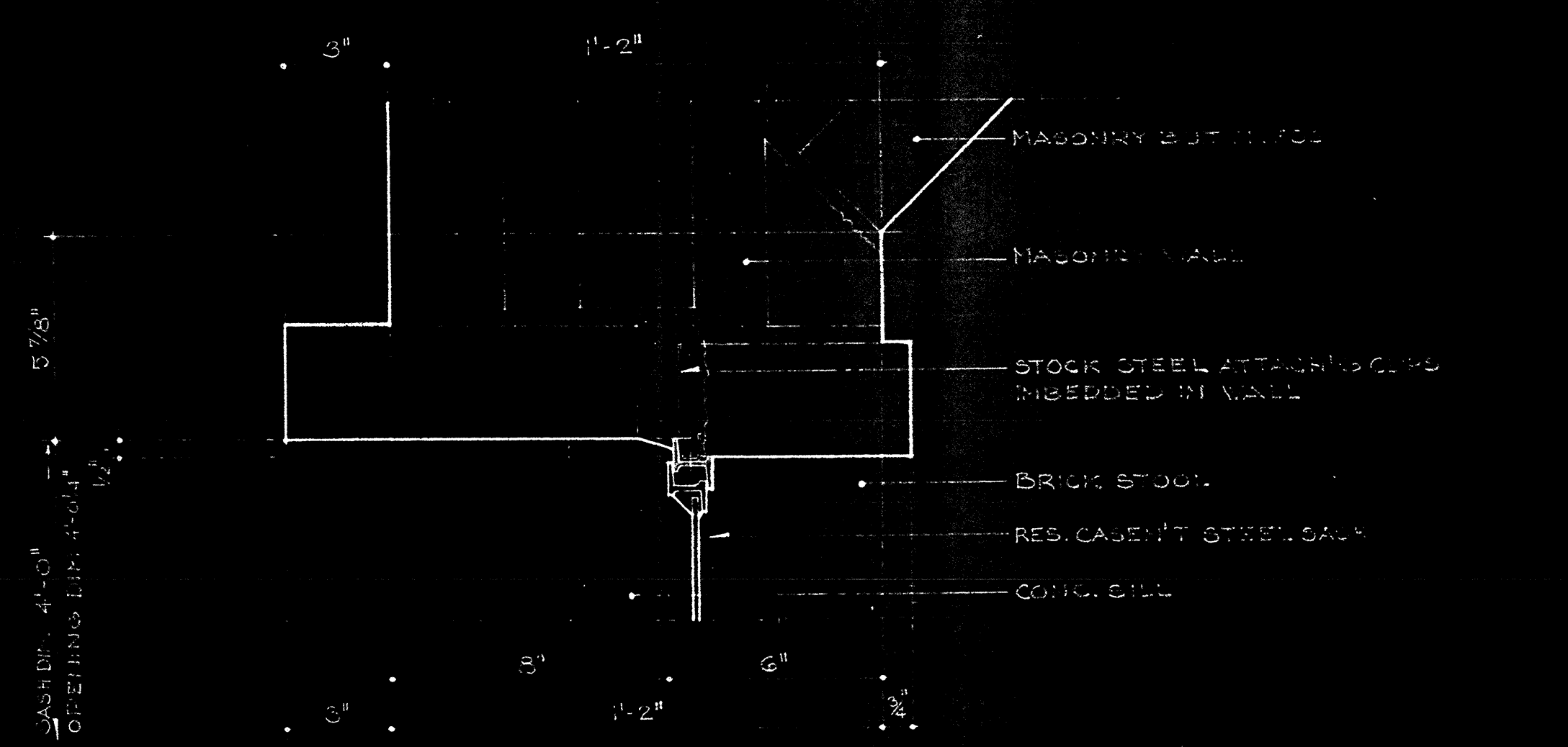
JAMB SCALE - 3/8" = 1'-0"
