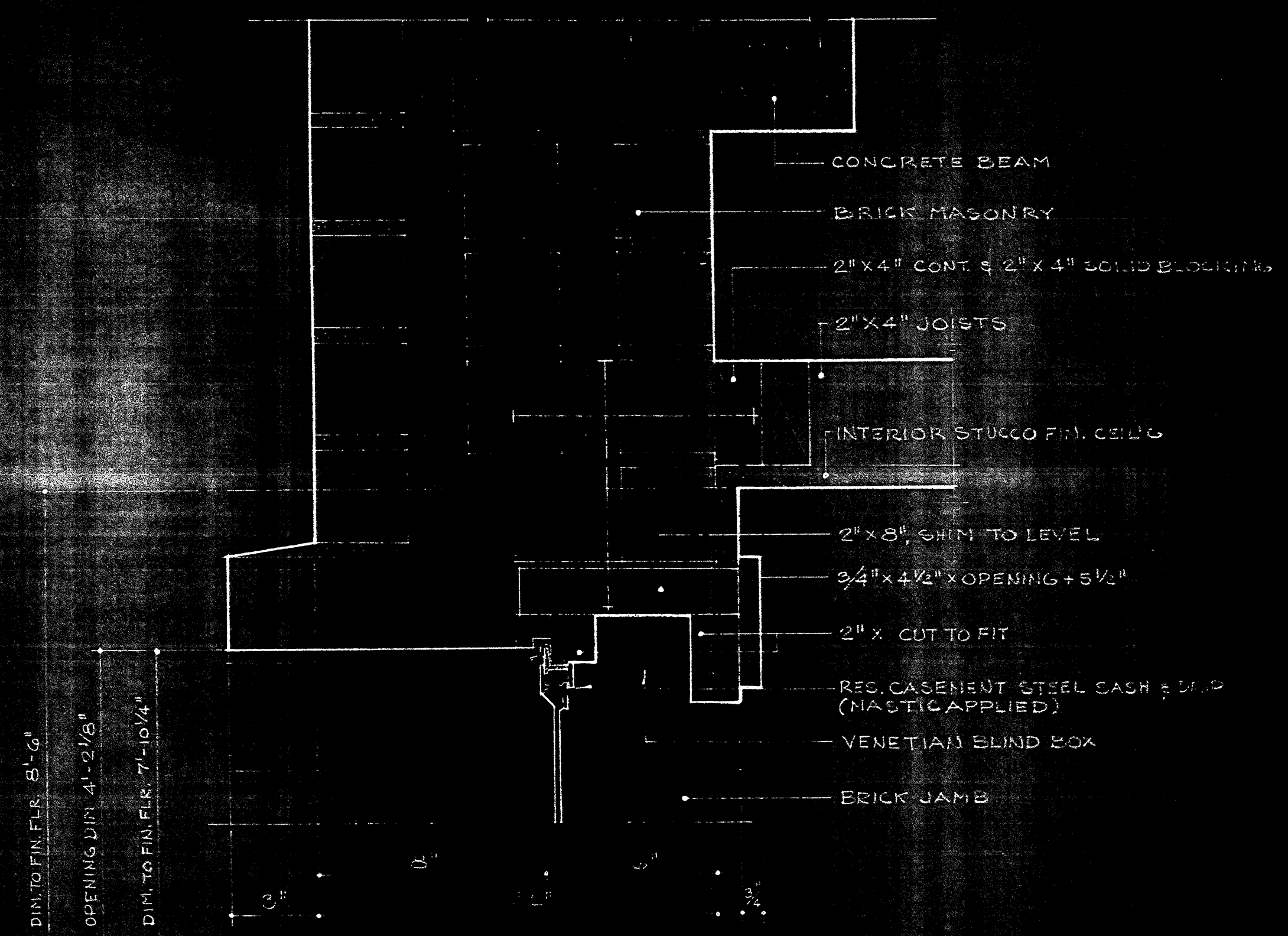
HEAD SCALE - 3/8" = 1'-0"
