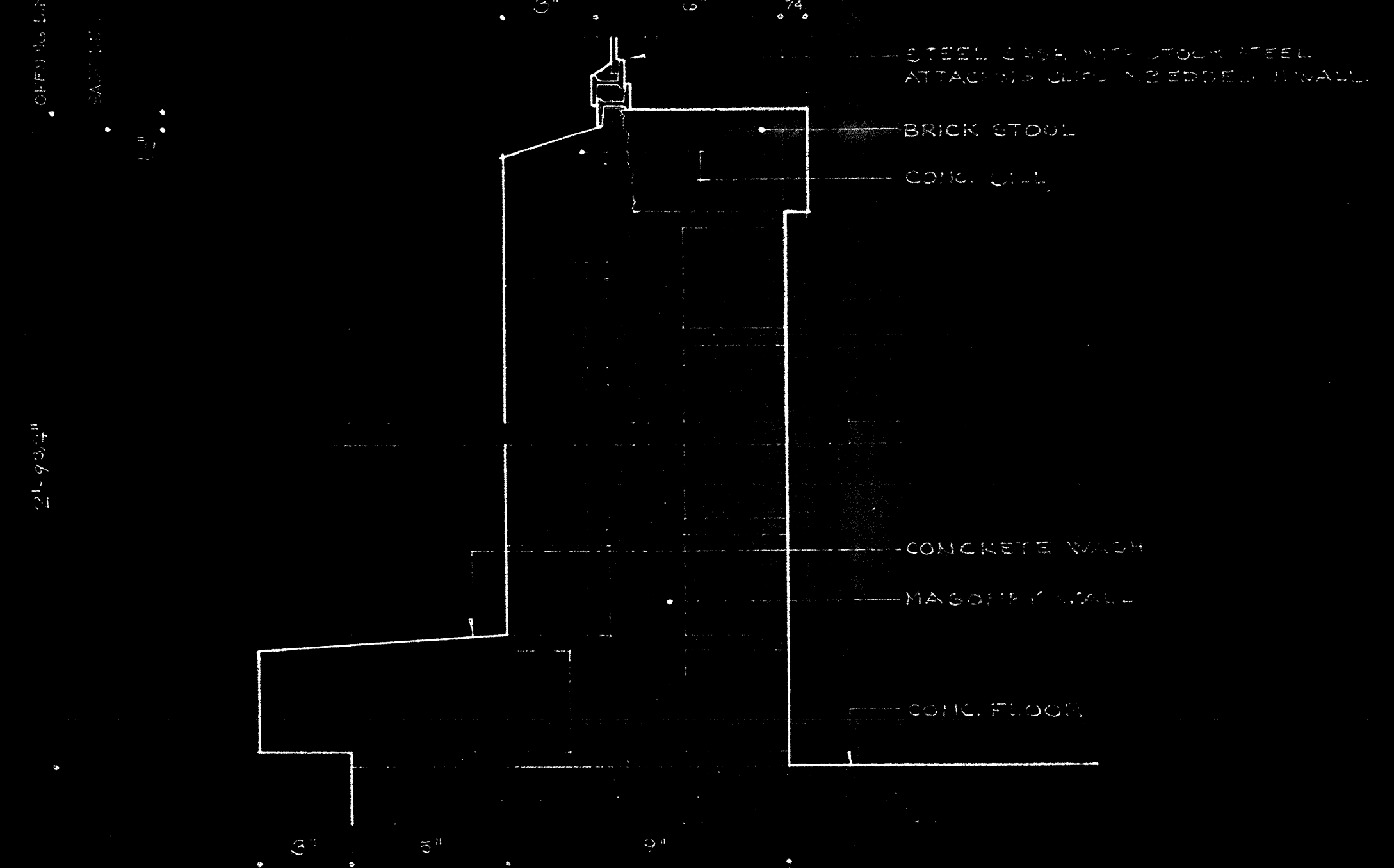
SILL SCALE - 3/8" = 1'-0"
