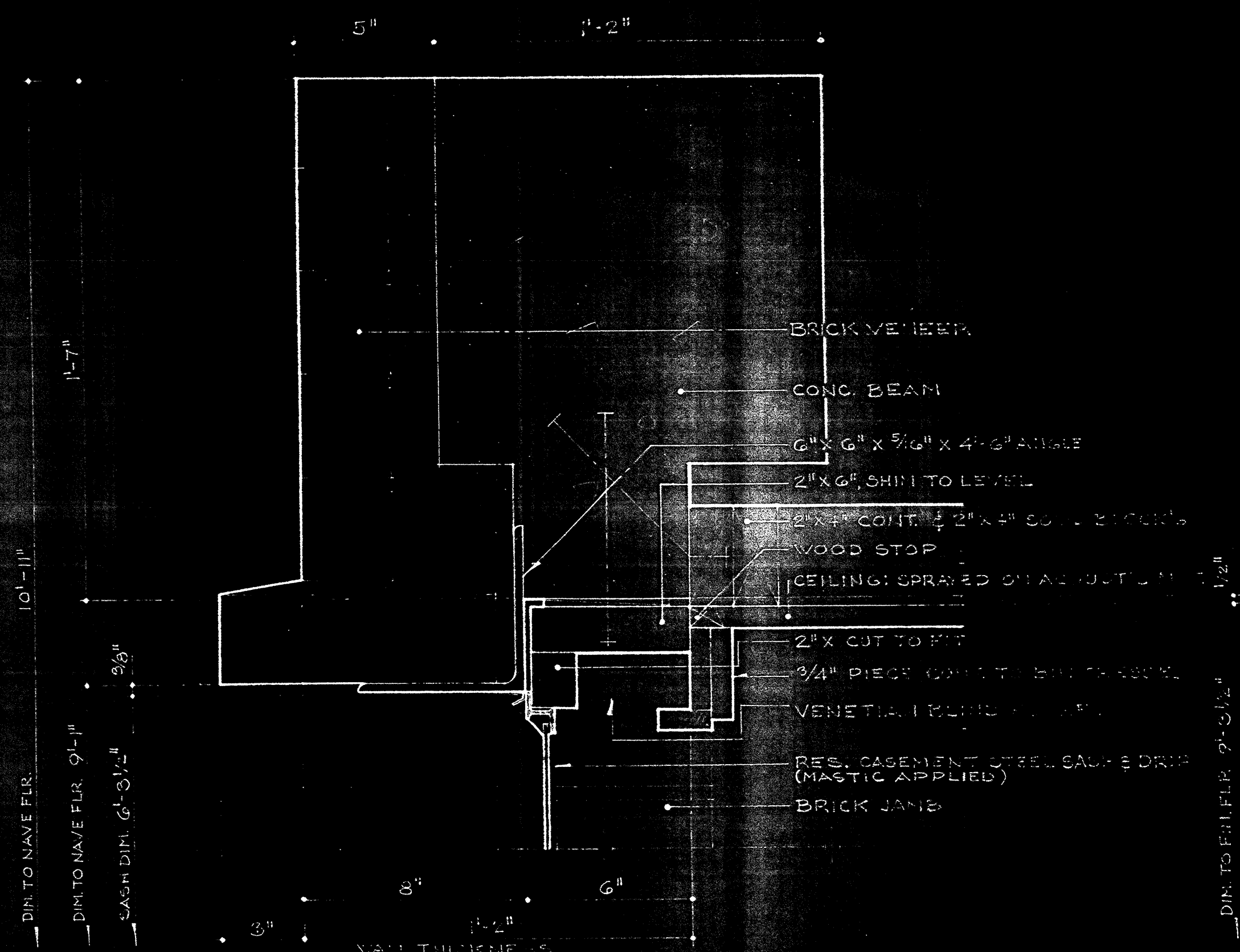
HEAD SCALE - 3/8" = 1'-0"
